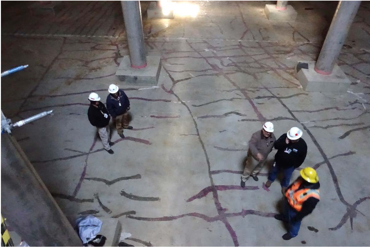
Fig. 5. Slab cracking, highlighted in purple from the dye used in the 2015 hydrostatic test adhering to epoxy that was gravity-fed into cracks (photograph from [7]).
